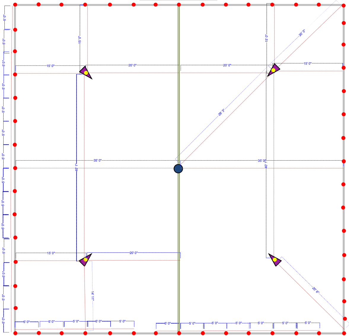
70' x 70' Pole Tent - Pole Placements
